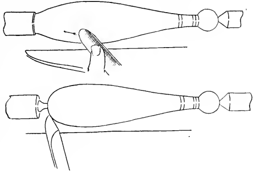
FIG. 316. LONG CONVEX CUTTING.
